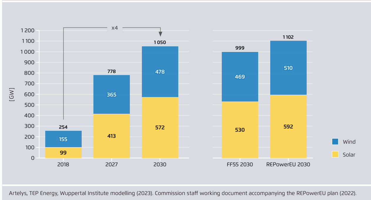
Installed capacity for solar and wind power in the EU Gas Exit scenario, Fit for 55 package and REPowerEU plan
