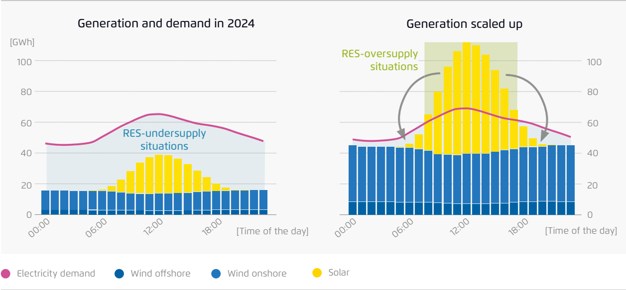
Hourly average generation and demand in Germany
