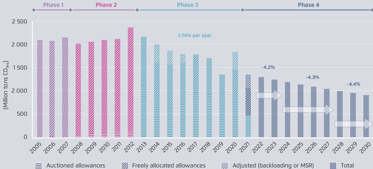
Allowances in the EU ETS (All countries, stationary installations and aviation)
