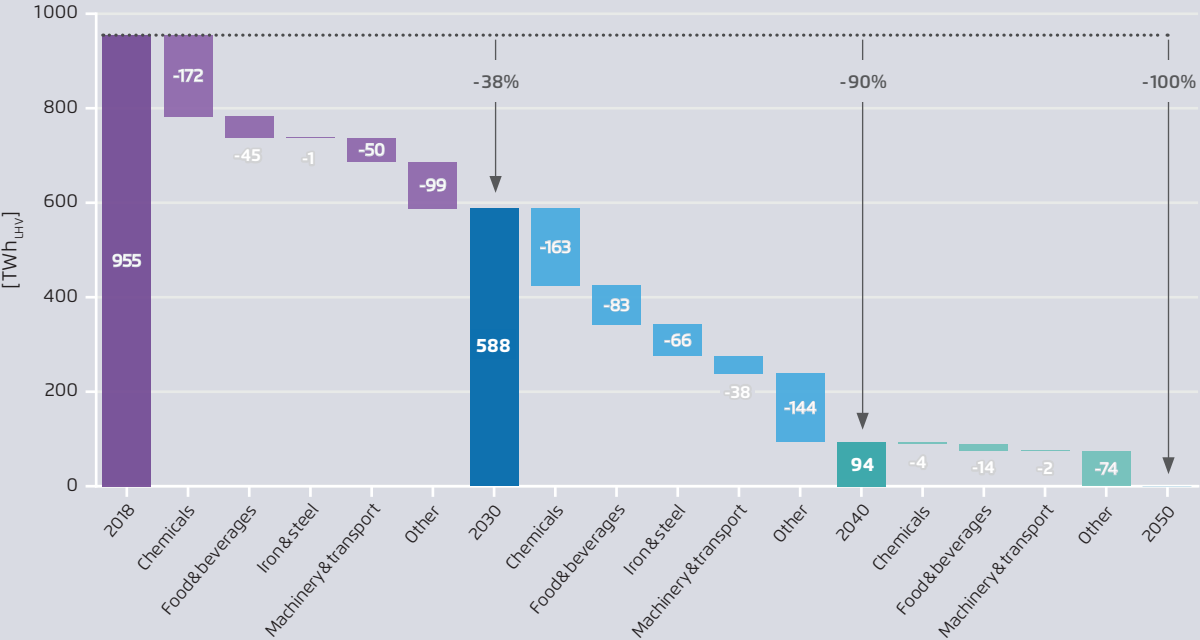
Evolution of total fossil gas consumption in the industry sector in the EU-27, 2018-2050
