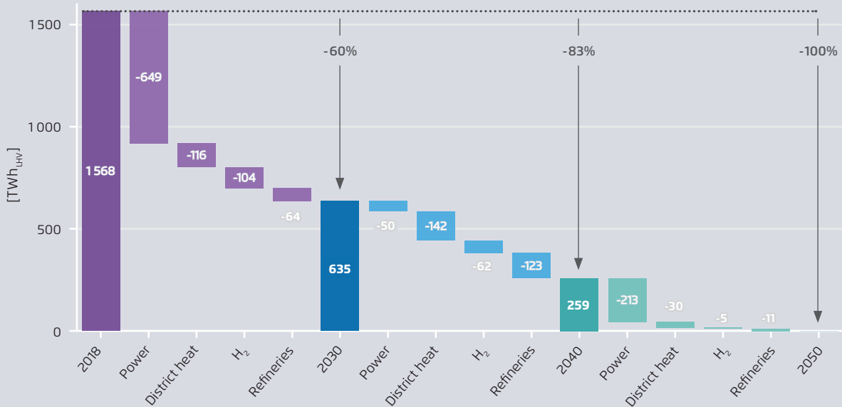
Evolution of total fossil gas consumption in the energy sector in the EU-27, 2018-2050
