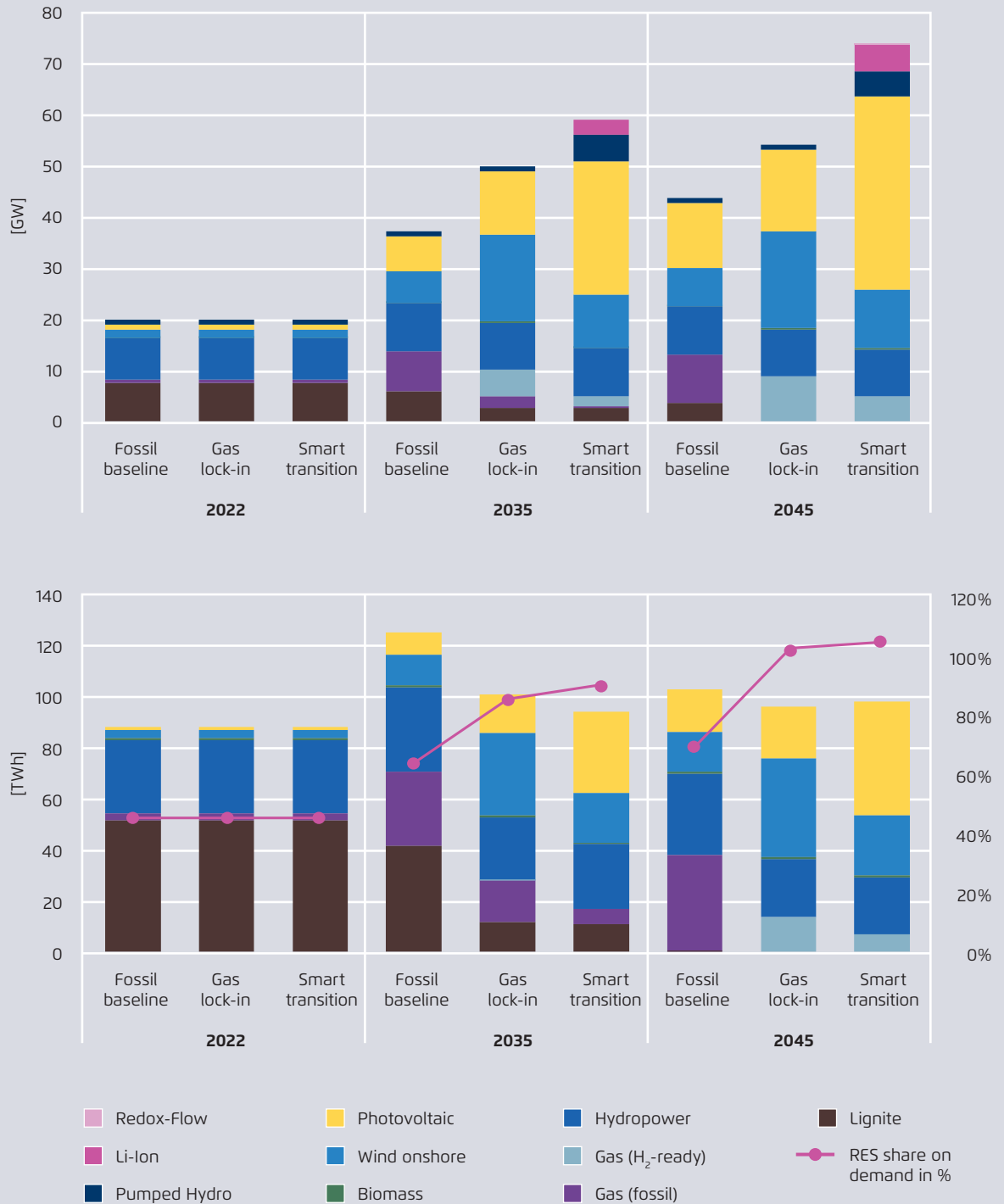
Installed capacities (top) and power generation (bottom) in 2022, 2035 and 2045 in the Western Balkans
