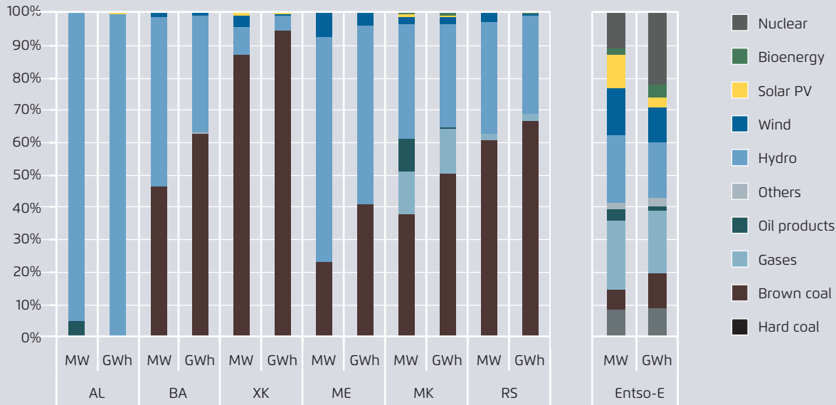
2018 power mix of WB-6 countries and ENTSO-E aggregate (relative terms)
