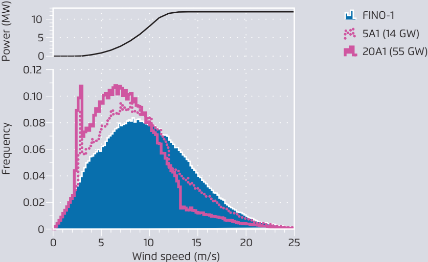
The 5A1 (red dotted line, 14 GW installed capacity) and the 20A1 (red solid line, 55 GW installed capacity) scenarios are compared with the climatology of wind speeds observed at the FINO-1 platform. Also shown for comparison at the top is the power curve for the assumed 12 MW turbine.
