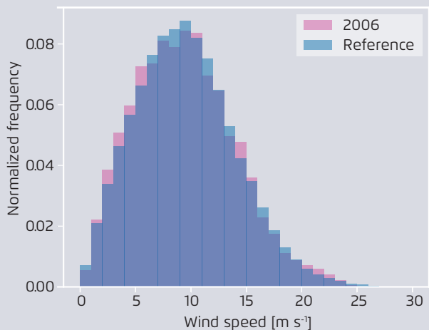
Comparison of distributions of wind speed (top left), wind direction (top right), and boundary layer stability (bottom) for the simulation year (2006) and the reference period
