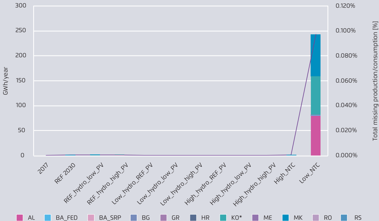
Missing production values (non-satisfied demand) for the sensitivity scenarios in GWh/year
