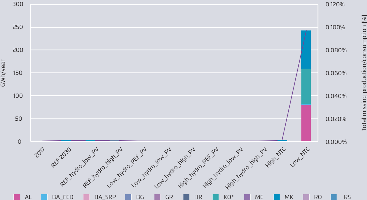
Missing production values (non-satisfied demand) for the sensitivity scenarios, GWh/year
