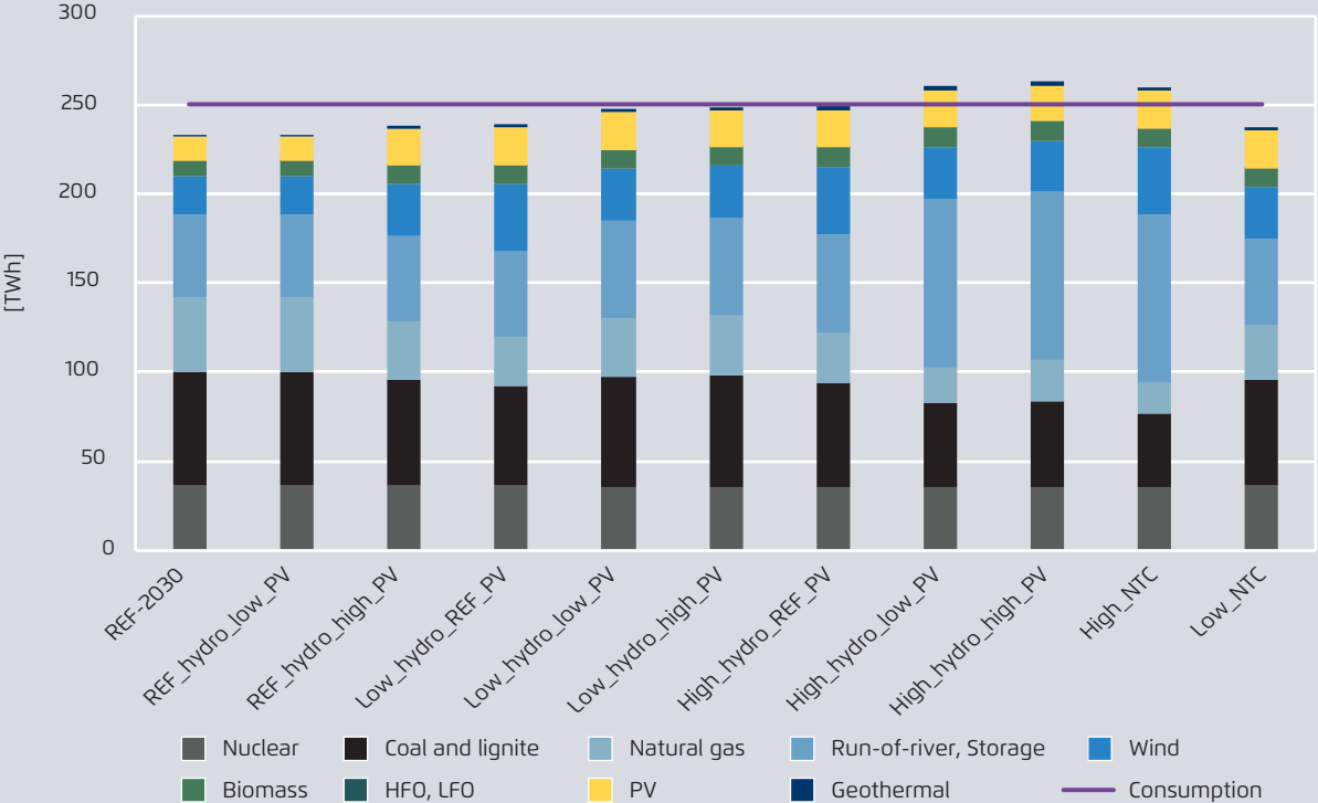
Electricity generation mix in SEE in all assessed scenarios, TWh/year
