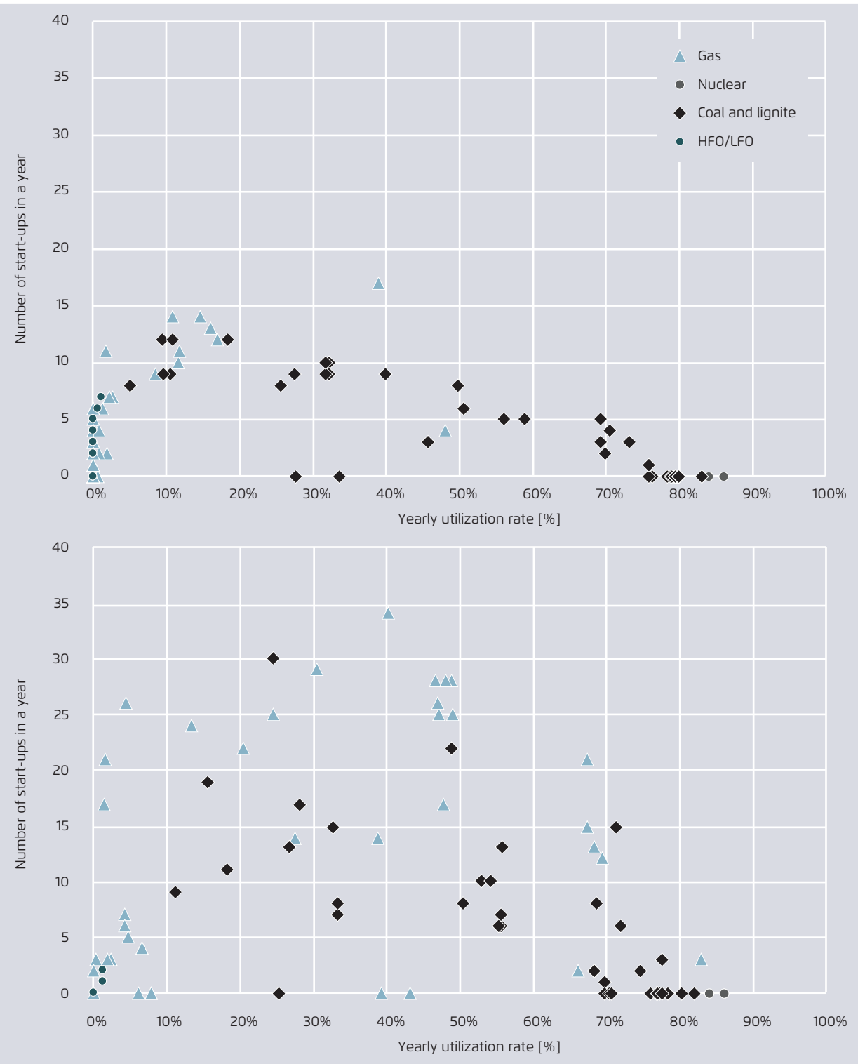
Yearly average utilization rates and number of start-ups (per year) on a unit level in the SEE region in 2017 (above) and 2030 (below)
