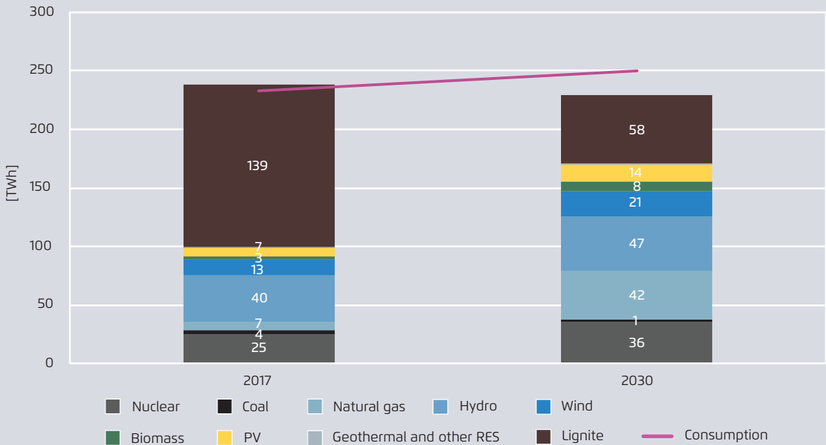
Electricity generation mix of the SEE region, 2017 (actual data) and 2030 (decarbonization scenario) Figure 2
