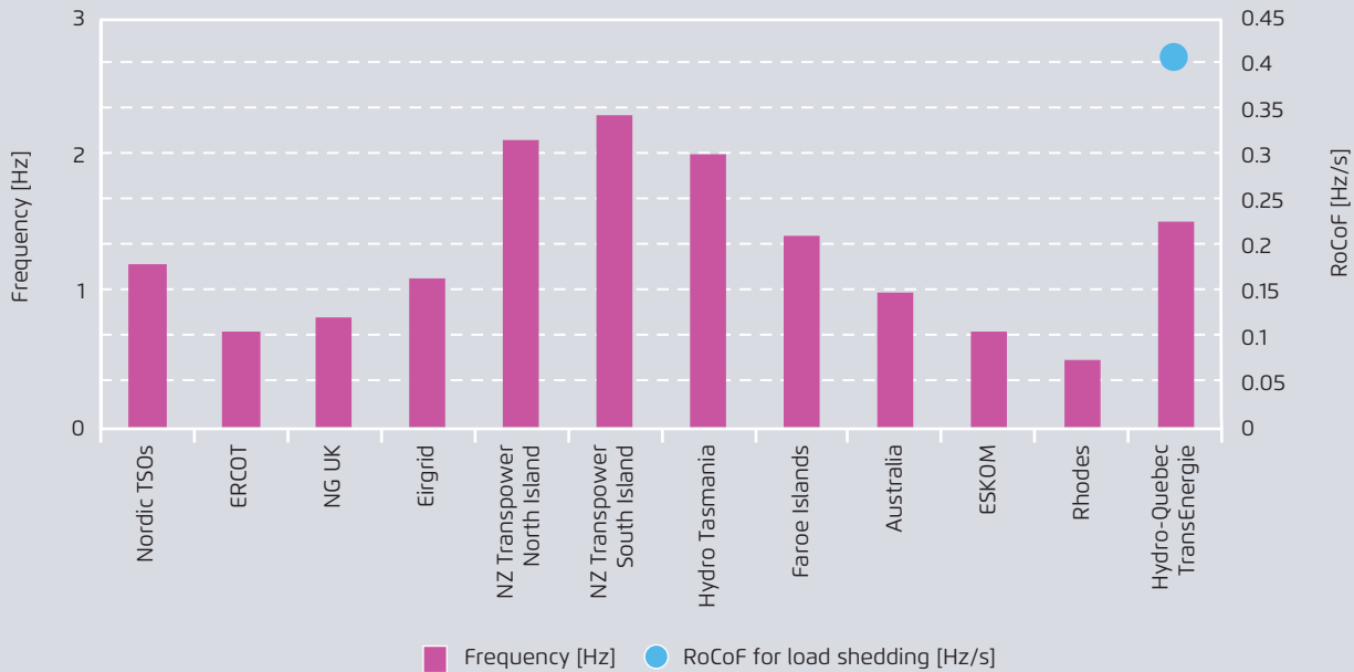
Frequency drop from nominal and RoCoF when load shedding starts for selected regions
