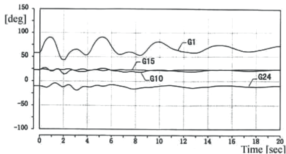
Generator internal Angle [deg]
