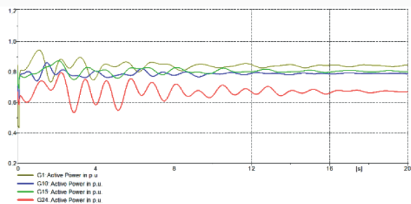
Generator active power output (Generator self capacity base) [p.u.]
