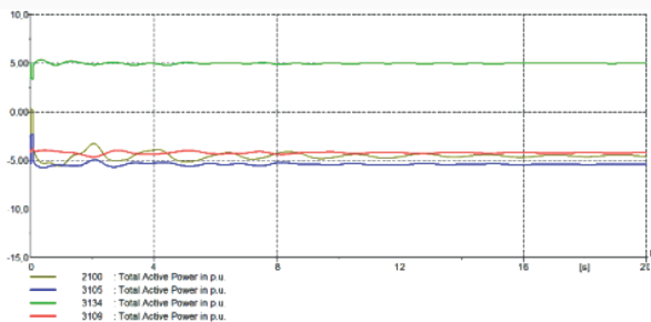
Line active power Flow [p.u.]
