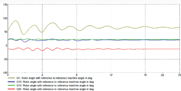
Generator internal Angle [deg]
