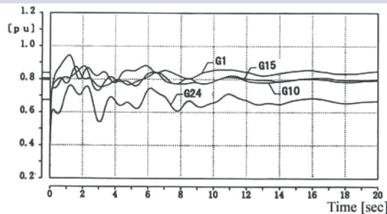
Generator active power output (Generator self capacity base) [p.u.]
