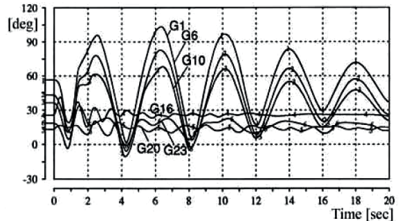
Generator internal Angle [deg]
