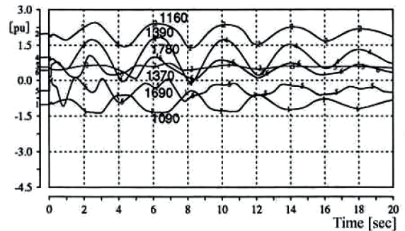
Line active power Flow [p.u.]
