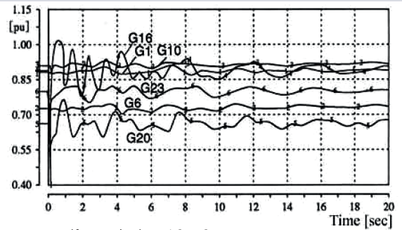
Generator active power output (Generator self capacity base) [p.u.]
