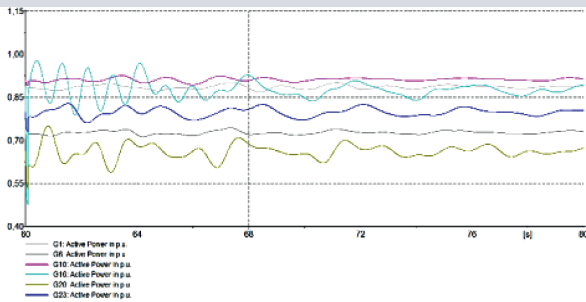
Generator active power output (Generator self capacity base) [p.u.]
