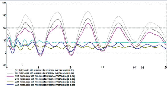
Generator internal Angle [deg]
