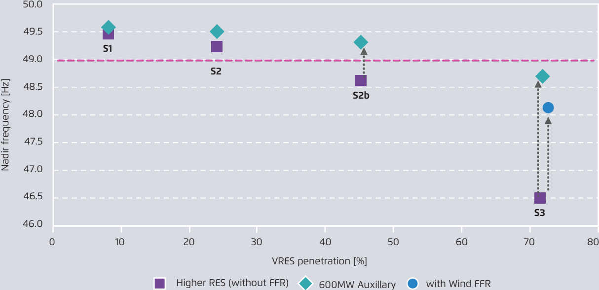
Nadir frequency and VRES penetration in eastern Japan with and without the 600MW ancillary service
