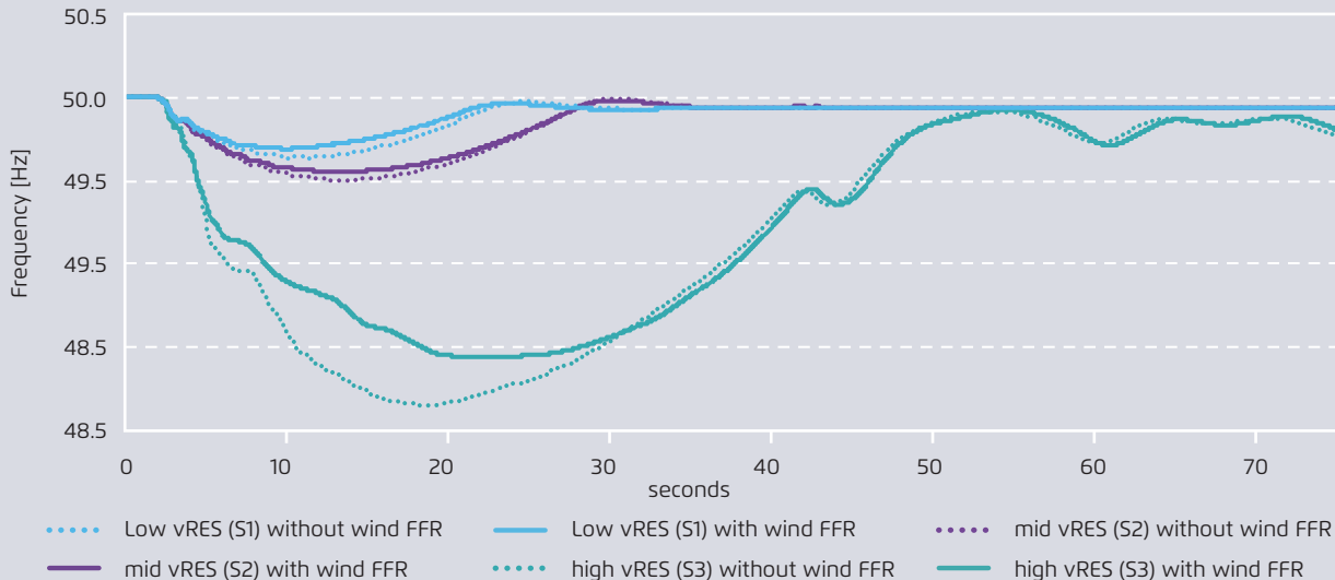
Frequency response after a 1,500 MW generation loss in eastern Japan in the government scenario
