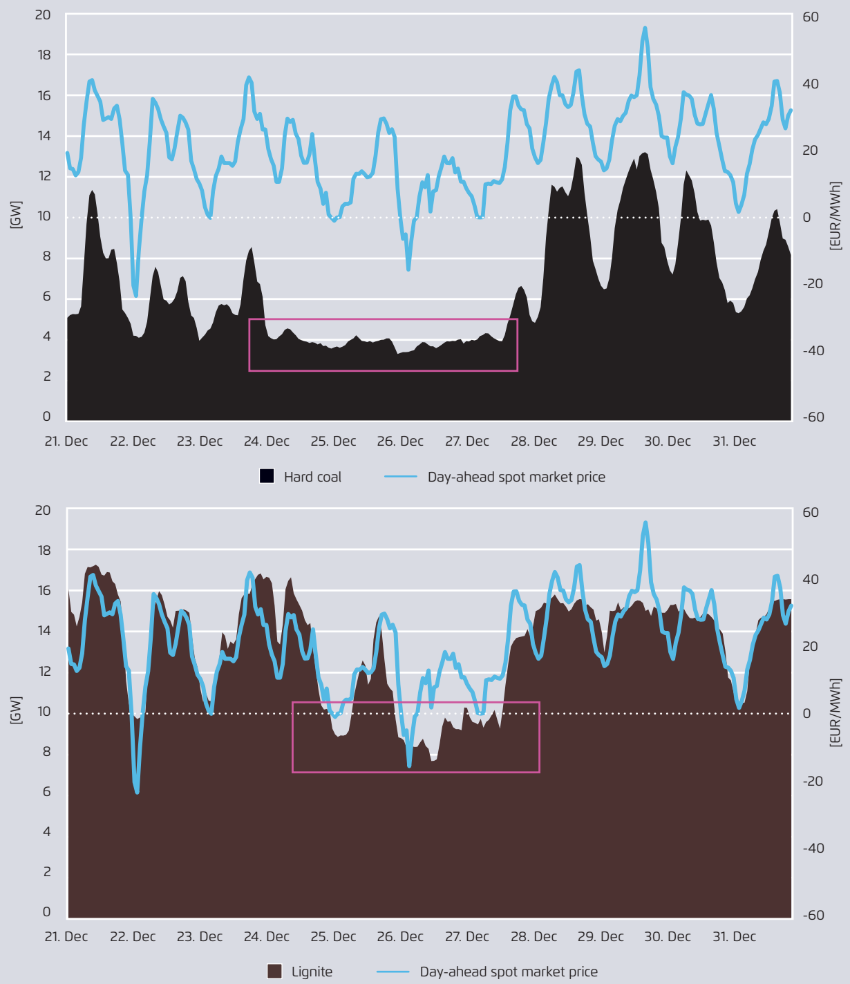
Electricity generation from hard-coal (top figure) and lignite plants (bottom figure) and day-ahead market prices, 21–31 Dec 2015. During this period, the minimum generation level of hard-coal plants amounted to 4 GW, whereas that of lignite plants amounted to 8 to 10 GW (as indicated by the highlights).
