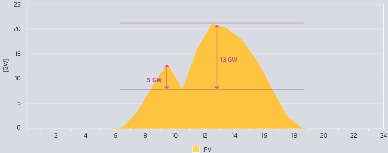
Electricity production of solar PV on 20 March 2015.
